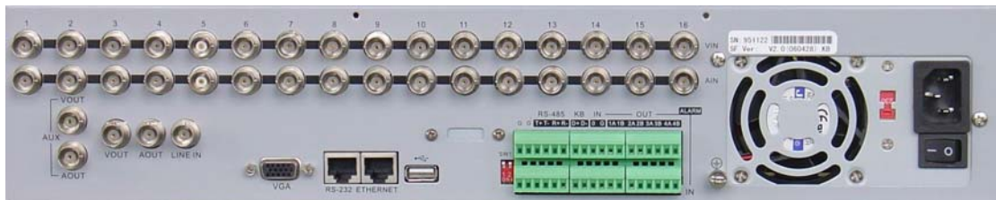
Rear Panel of DS-8016HFI-S
